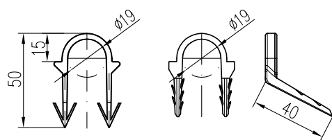
type A
