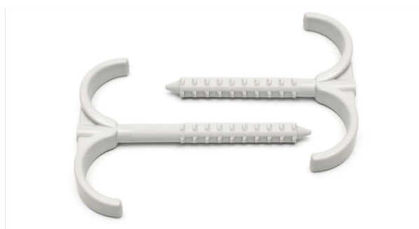
N 2032 8/75 • N 2032 8/95
