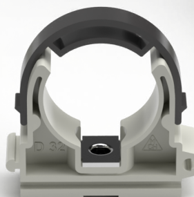
Bracket with shackle and M6 metal nut
