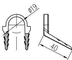
type B
