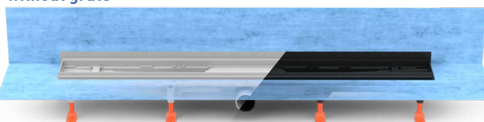
Linear drain D40 against the wall with waterproofing, without grate
