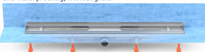
Linear drain D40 against the wall with SS frame and waterproofing, without grate
