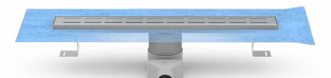
Stainless steel linear drain D50 with waterproofing membrane and height-adjustable swivel siphon
