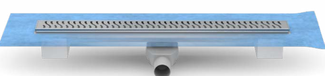
Linear floor drain D50 with waterproofing membrane, stainless steel frame and swivel siphon
