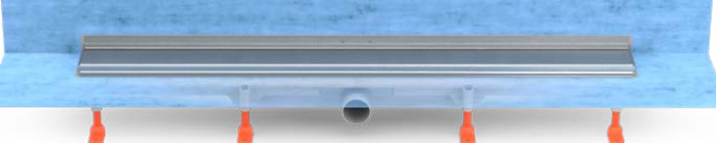
Linear floor drain D40 against the wall side outlet, with waterproofing membrane and stainless steel frame
